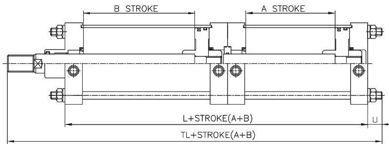
(Applied with aluminum tube \varnothing 125 \sim \varnothing 200 )
