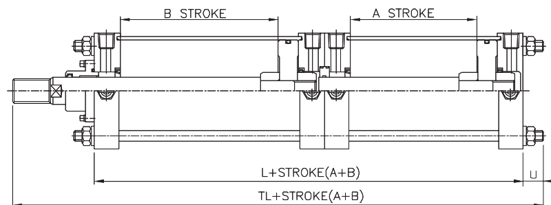
(Applied iron tube \varnothing 180 \sim \varnothing 300 )
