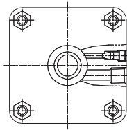
(Applied with aluminum tube \varnothing 125 \sim \varnothing 200 )
